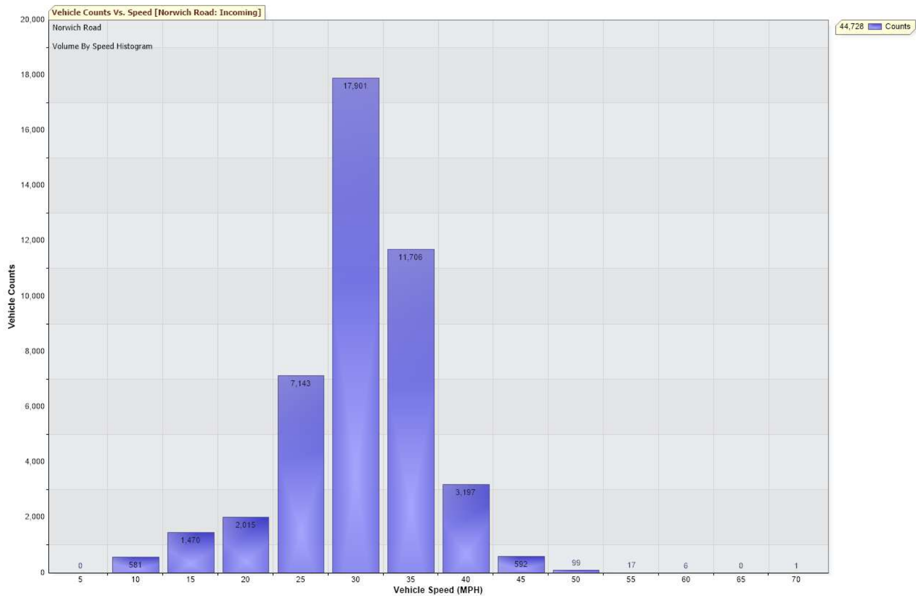
Chart to show vehicle count v speed at Norwich Road between 7 & 29 July 2026
