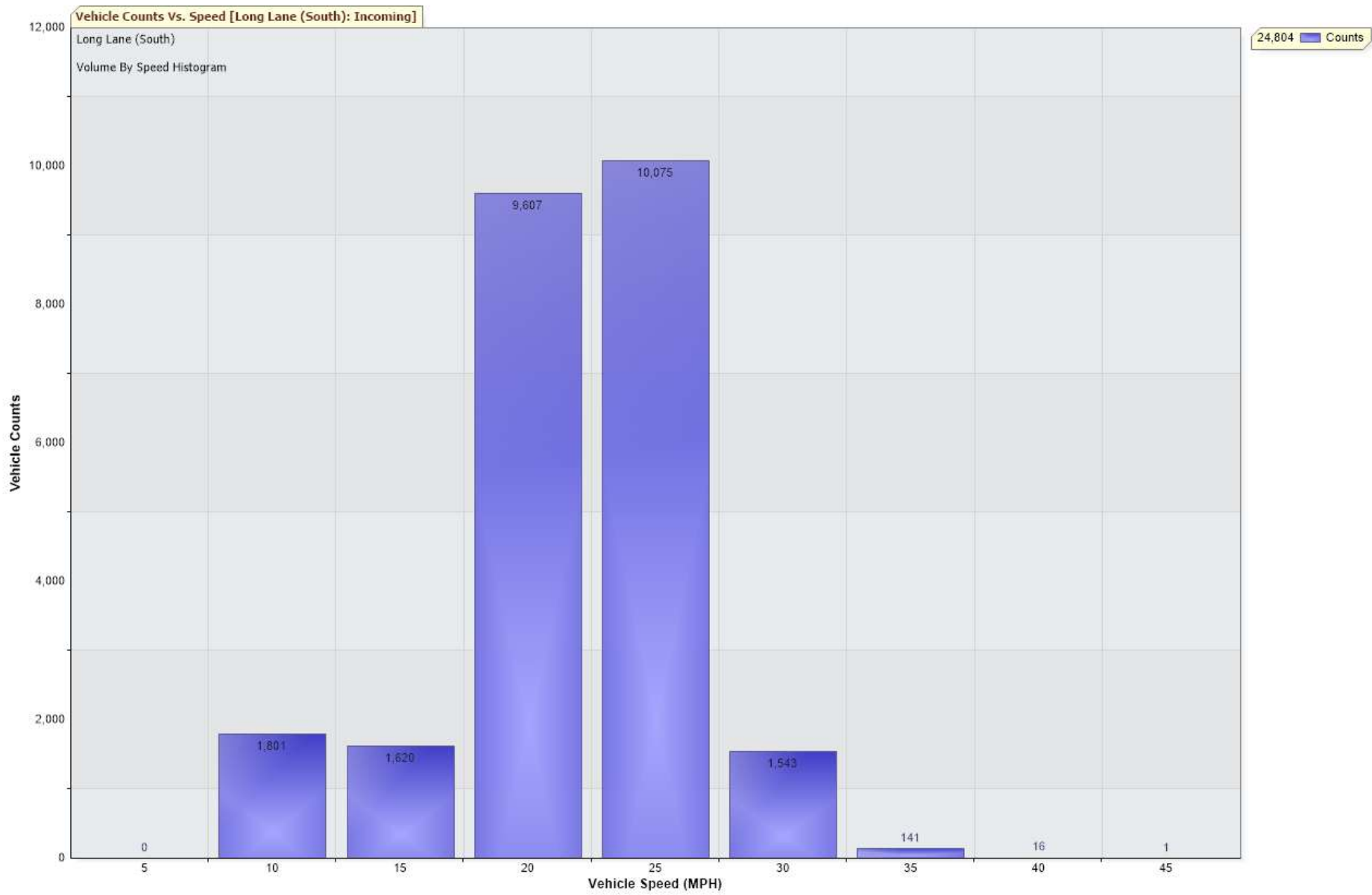
Chart to show vehicle count v speed at Long Lane (South) between 11 and 28 June 2026
