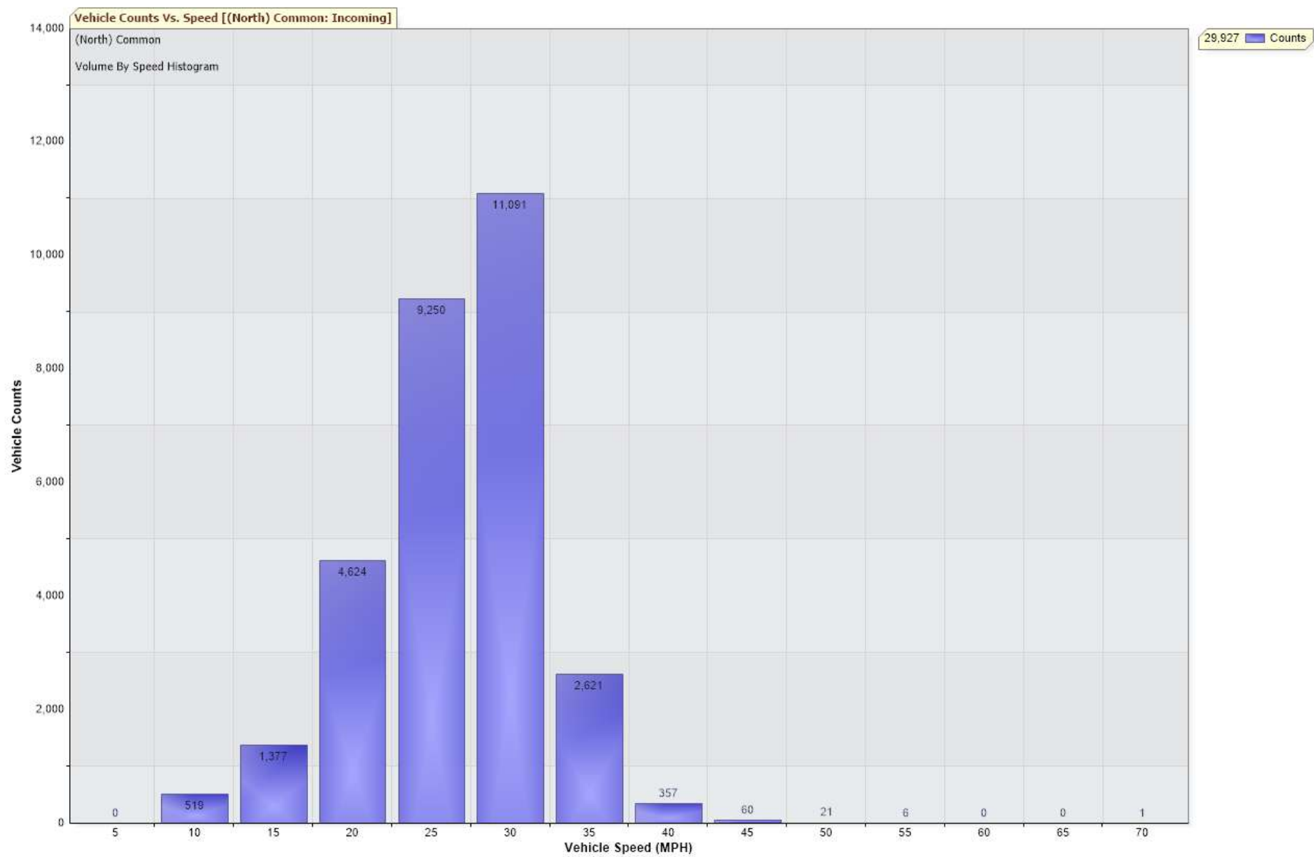
Chart to show vehicle count v speed at Common (north) between 2 and 21 Dec 2025
