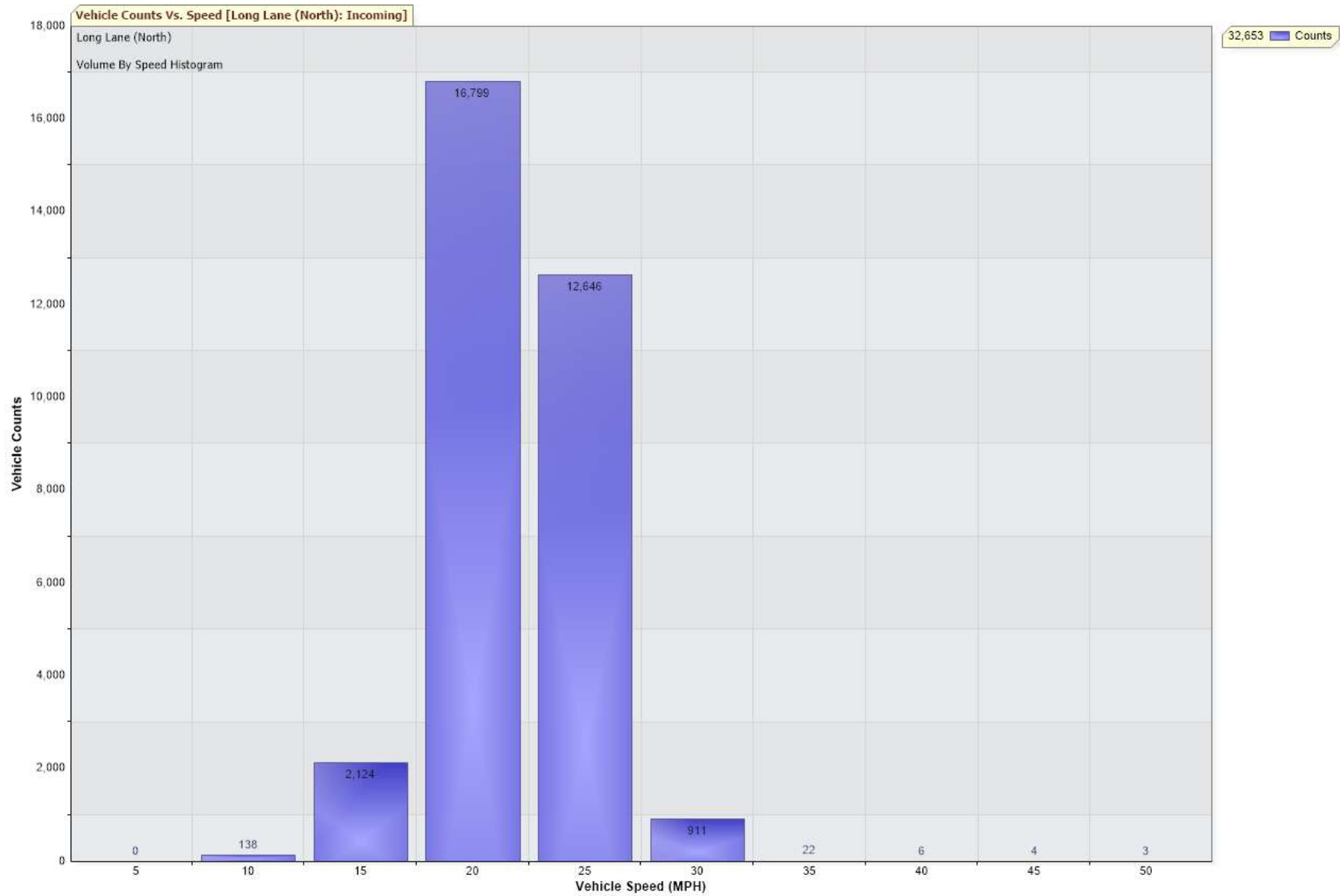
Chart to show vehicle count v speed at Long Lane (North facing) between 8 Sep and 3 Oct 2025
