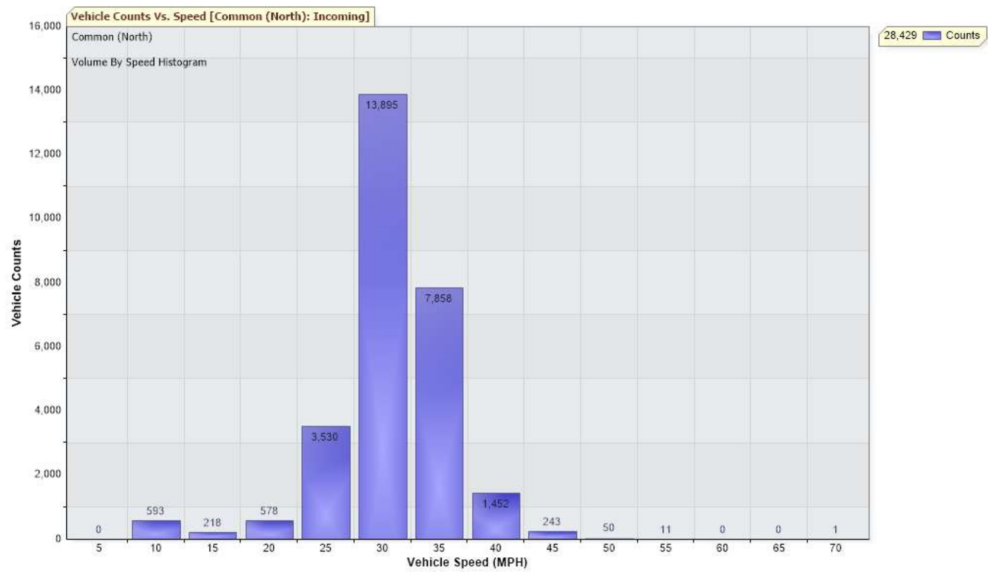
Chart to show vehicle count v speed at The Common (North) between 14 May and 2 June 2025
