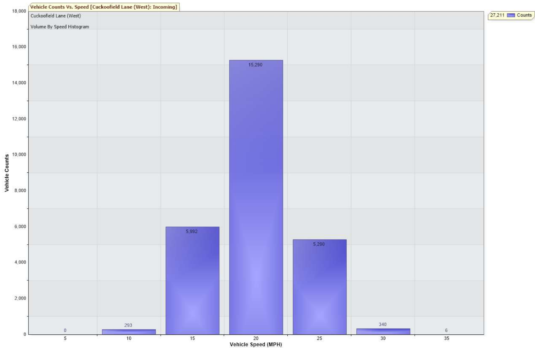
Chart to show vehicle count v speed at Cuckoofield Lane (west) between 6 & 25 October 2025
