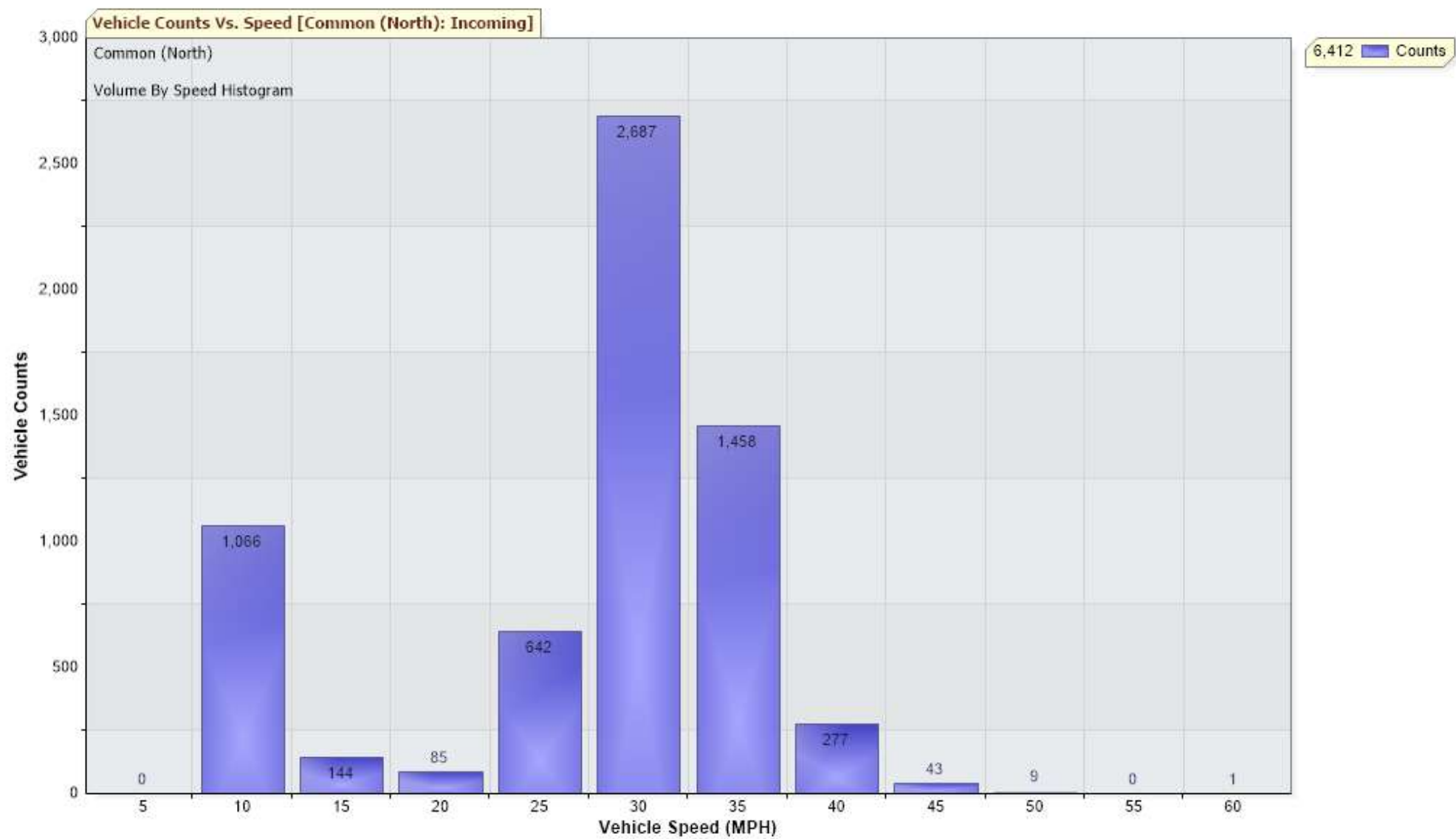
Chart to show vehicle count v speed at Common (north) between 18 and 22 July 2025
