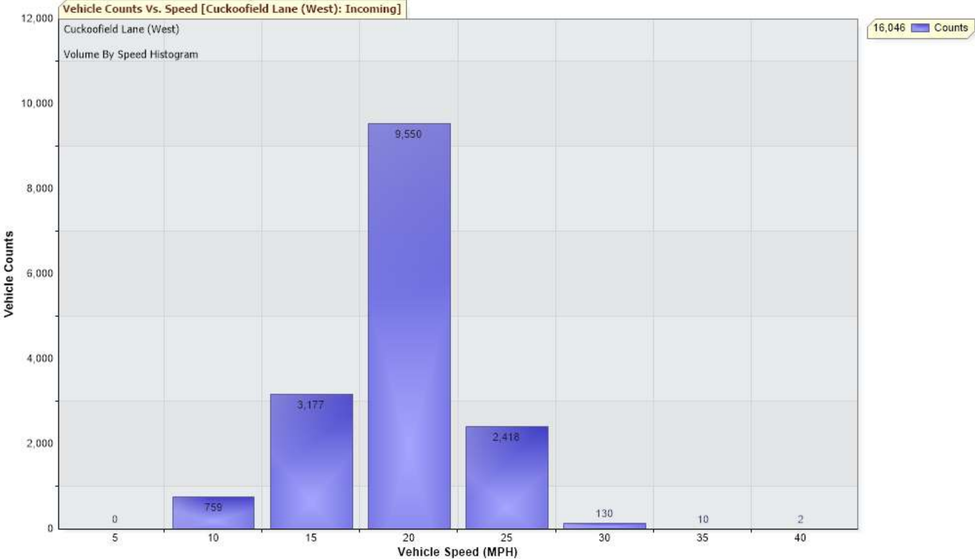
Chart to show vehicle count v speed at Cuckoofield Lane (West) between 14 and 29 April 2025
