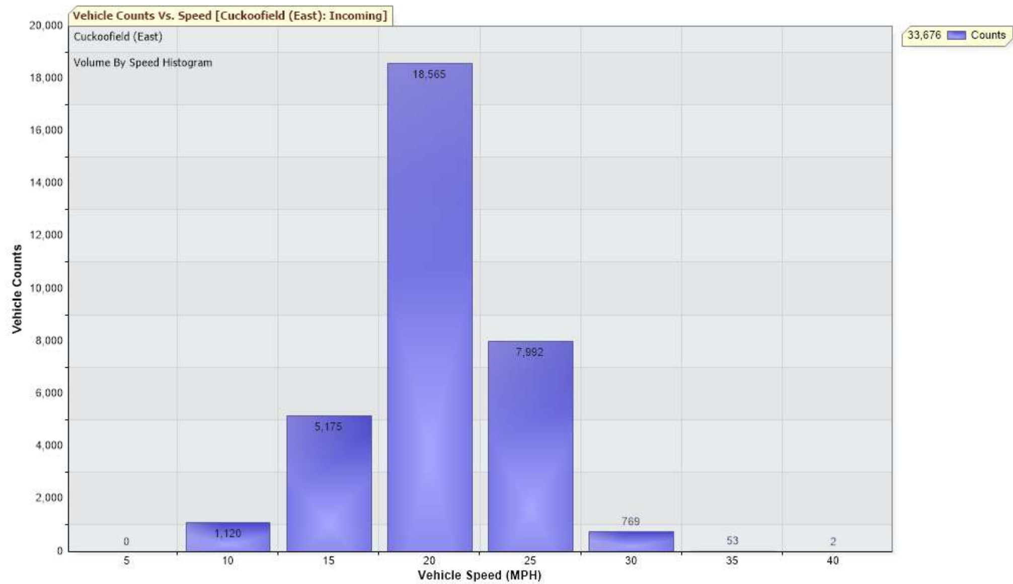
Chart to show vehicle count v speed at Cuckoofield Lane (East) between 15 Aug & 3 Sep 2025
